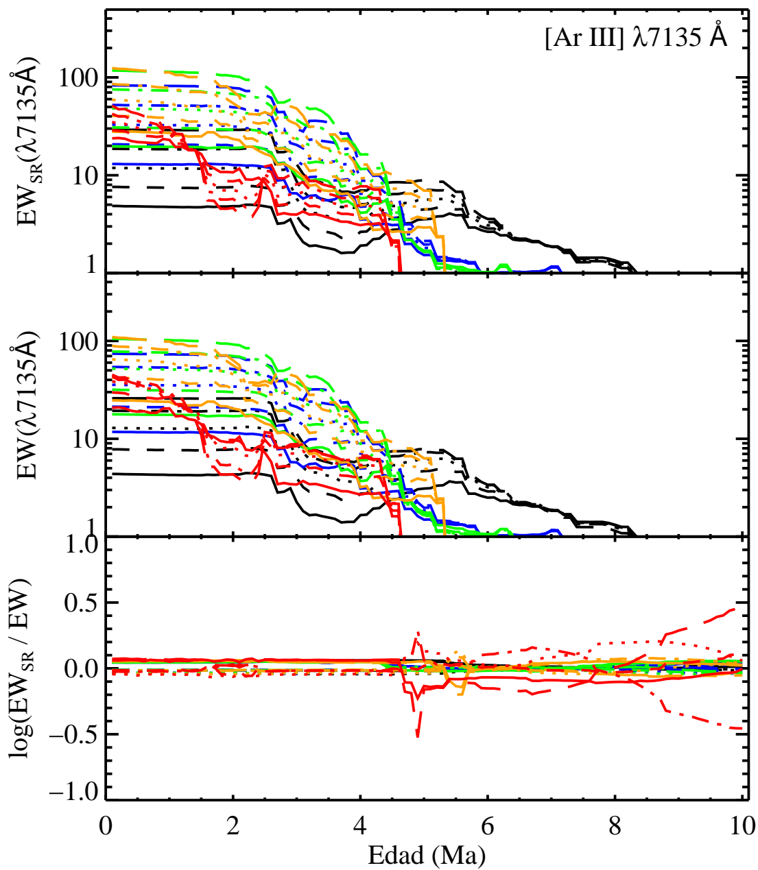
FIGURA C.22: EW_{SR} , EW y \log \frac{EW_{SR}}{EW} para [\text{Ar III}] \lambda 7135 \text{ \AA} .
