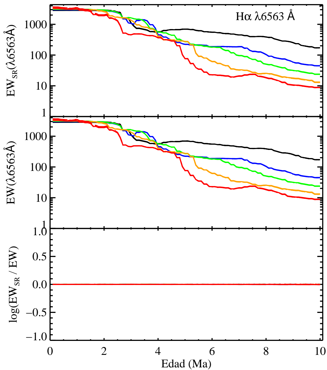
FIGURA C.17: EW_{SR} , EW y \log \frac{EW_{SR}}{EW} para H \alpha .
