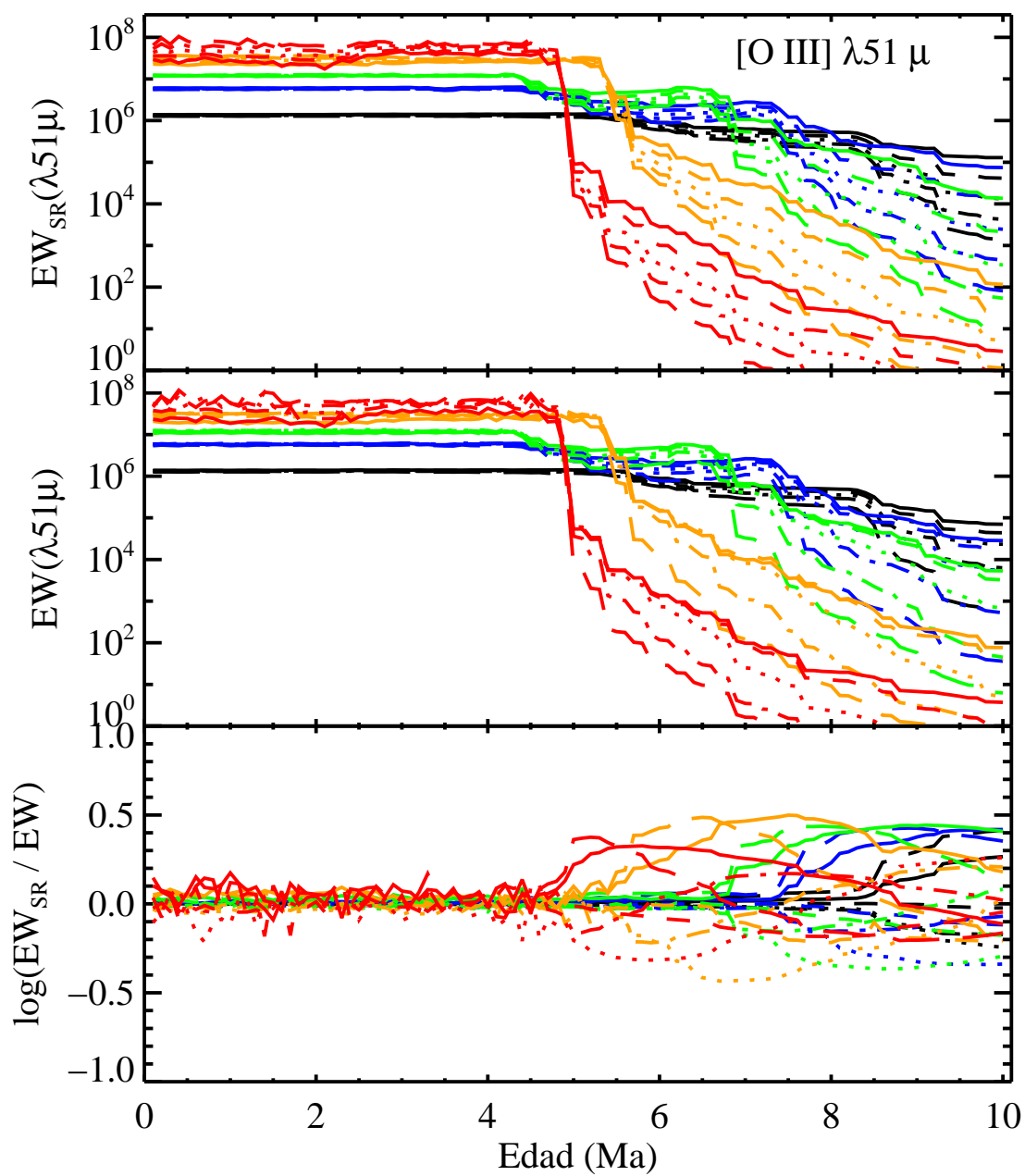
FIGURA C.35: EW_{SR} , EW y \log \frac{EW_{SR}}{EW} para [O III] \lambda 51 \mu .
