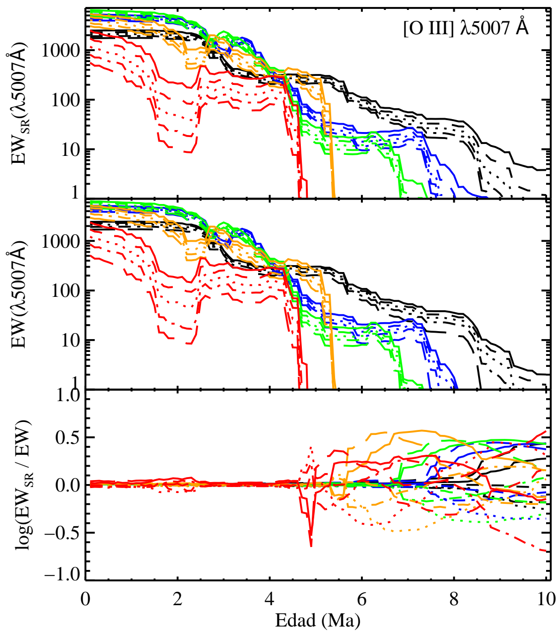
FIGURA C.12: EW_{SR} , EW y \log \frac{EW_{SR}}{EW} para [O III] \lambda 5007 Å.
