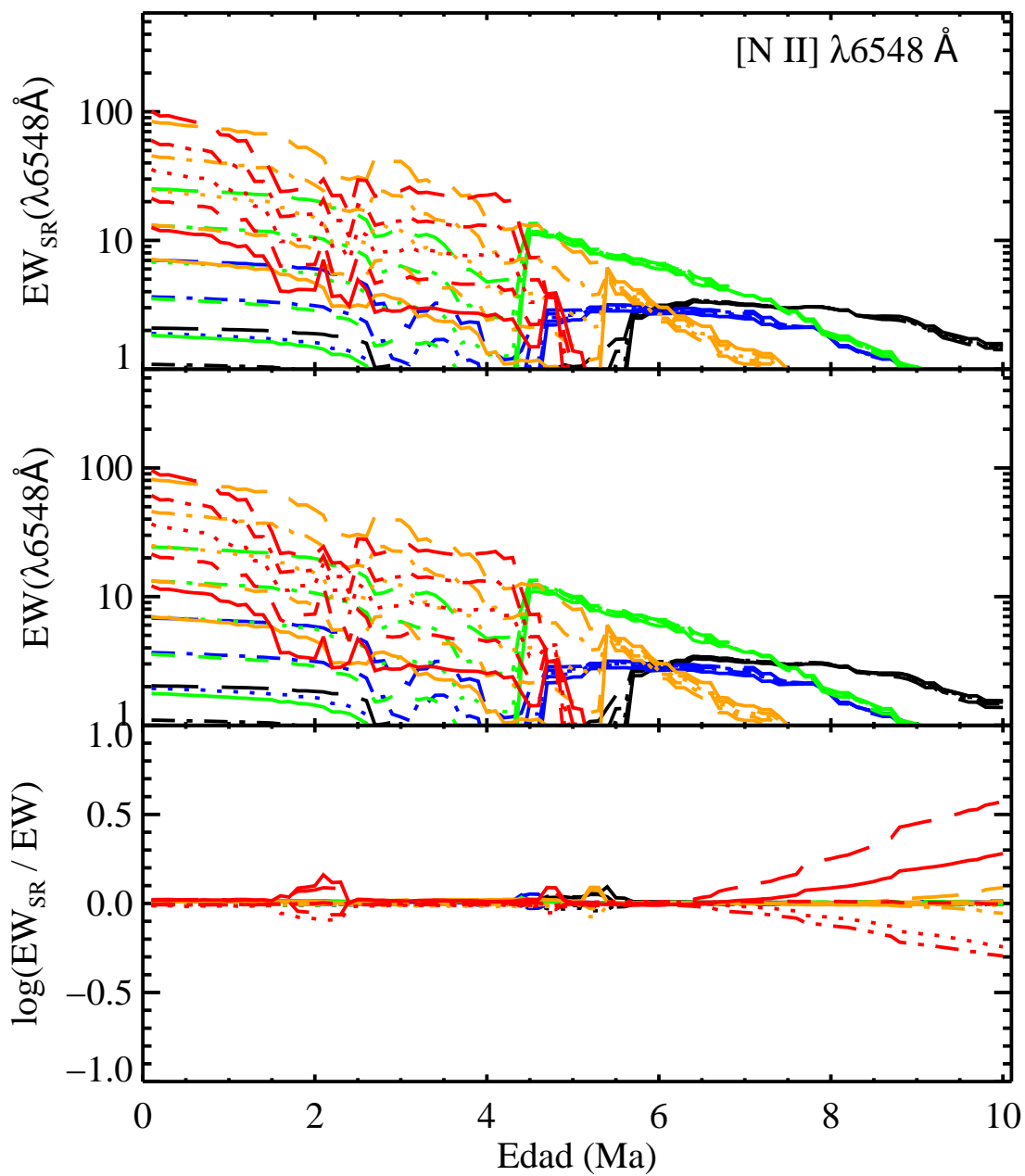
FIGURA C.16: EW_{SR} , EW y \log \frac{EW_{SR}}{EW} para [N II] \lambda 6548 Å.
