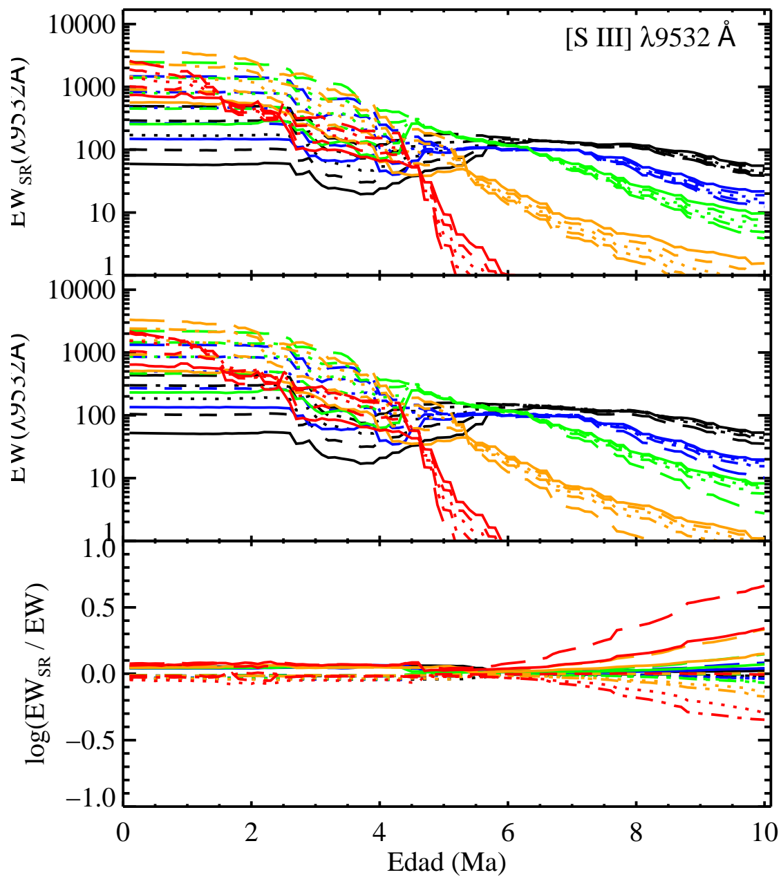
FIGURA C.26: EW_{SR} , EW y \log \frac{EW_{SR}}{EW} para [S III] \lambda 9532 Å.
