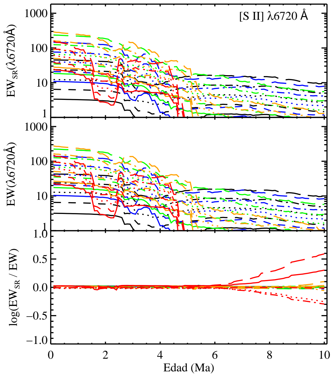
FIGURA C.20: EW_{SR} , EW y \log \frac{EW_{SR}}{EW} para [S II] \lambda 6720 \text{ \AA} .
