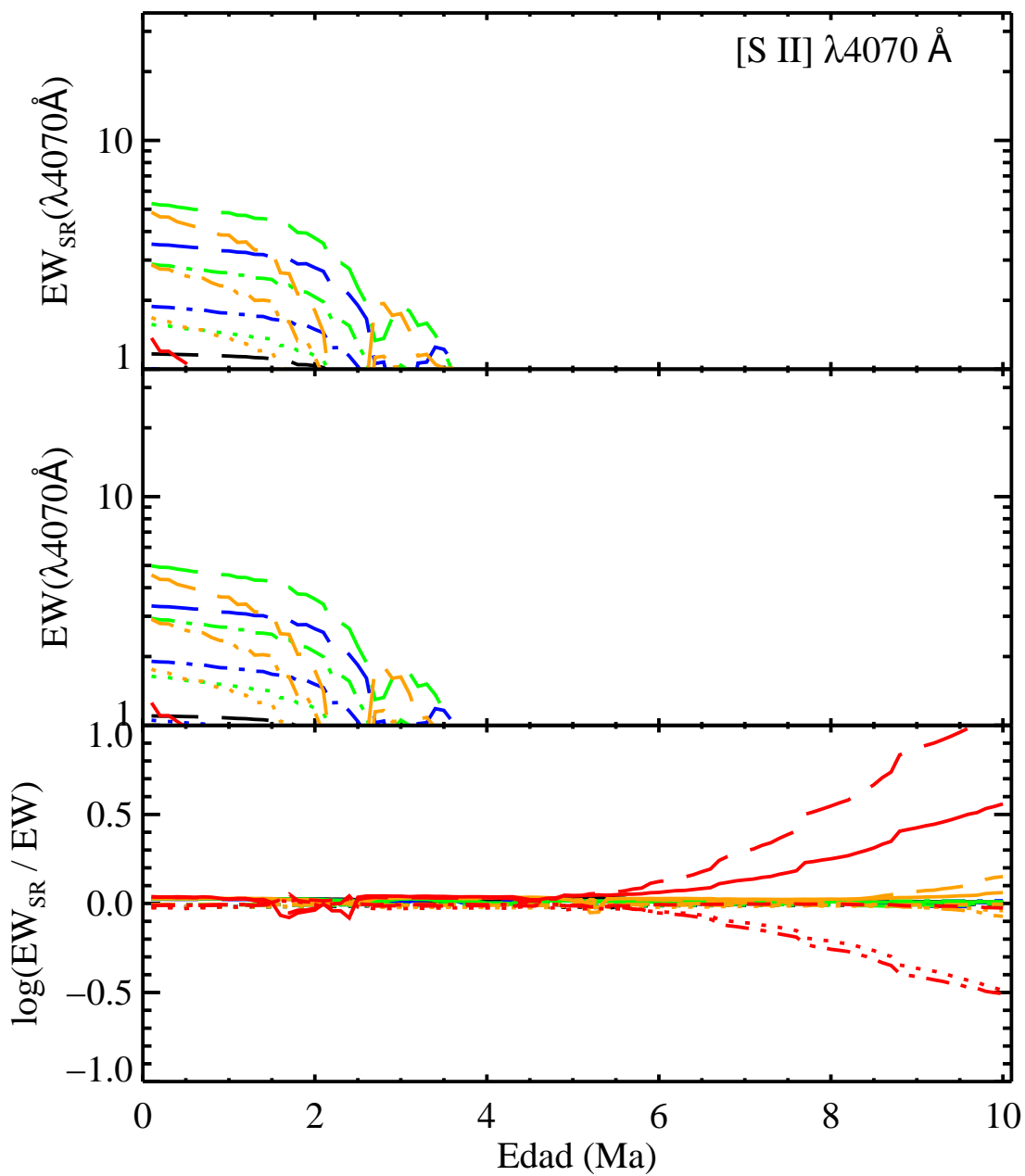
FIGURA C.6: EW_{SR} , EW y \log \frac{EW_{SR}}{EW} para [S II] \lambda 4070 Å.
