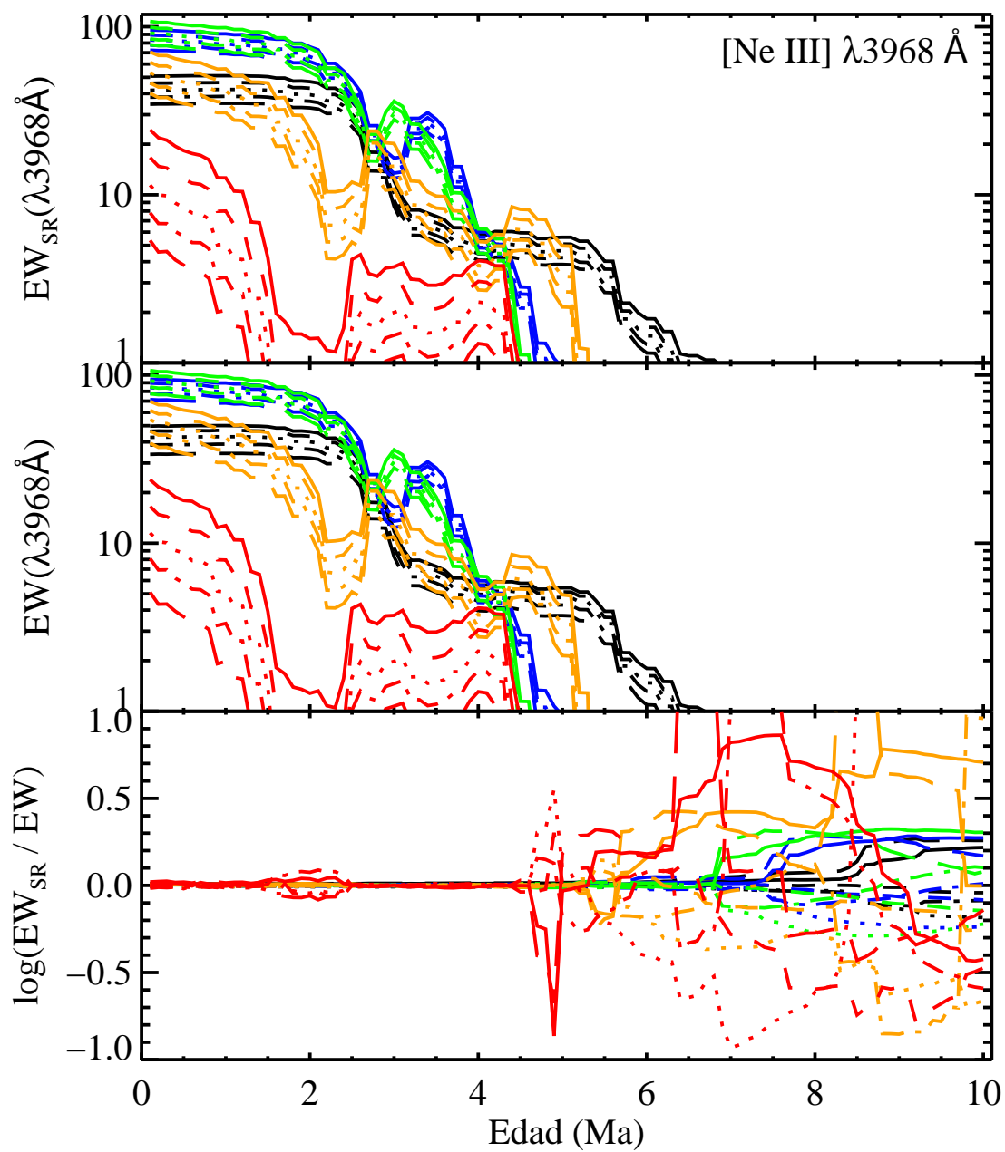
FIGURA C.5: EW_{SR} , EW y \log \frac{EW_{SR}}{EW} para [\text{Ne III}] \lambda 3968 \text{ \AA} .
