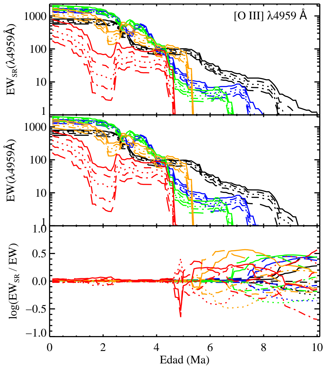
FIGURA C.11: EW_{SR} , EW y \log \frac{EW_{SR}}{EW} para [O III] \lambda 4959 Å.
