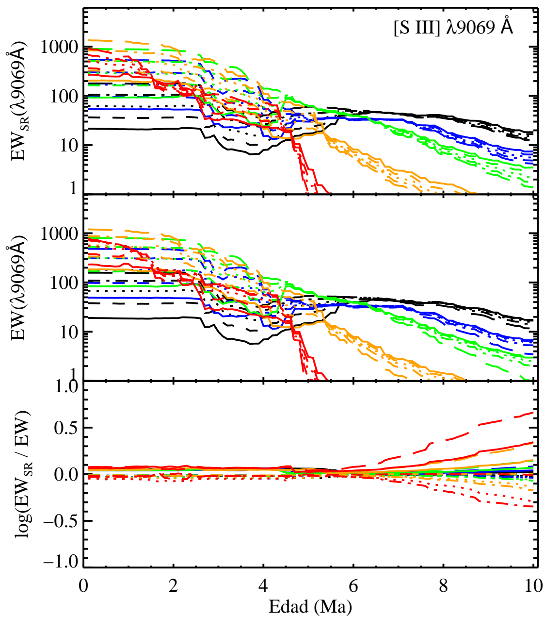
FIGURA C.25: EW_{SR} , EW y \log \frac{EW_{SR}}{EW} para [S III] \lambda 9069 Å.
