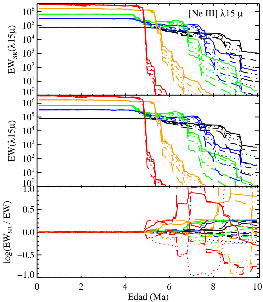
FIGURA C.31: EW_{SR} , EW y \log \frac{EW_{SR}}{EW} para [Ne III] \lambda 15 \mu .
