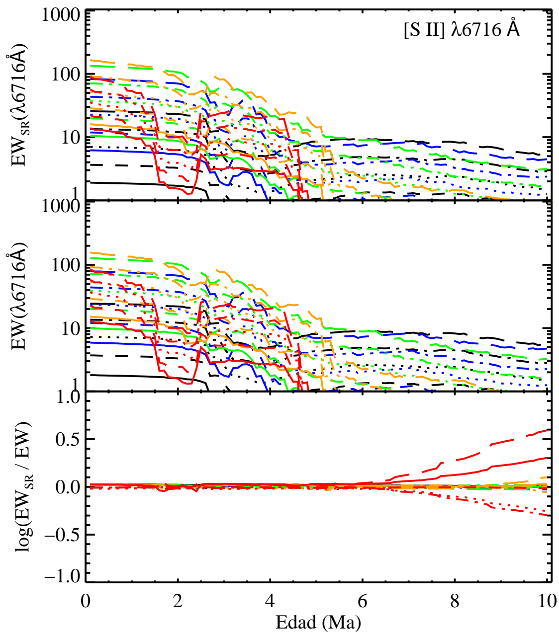
FIGURA C.19: EW_{SR} , EW y \log \frac{EW_{SR}}{EW} para [S II] \lambda 6716 \text{ \AA} .
