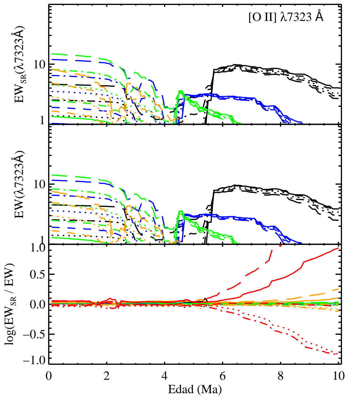
FIGURA C.23: EW_{SR} , EW y \log \frac{EW_{SR}}{EW} para [O II] \lambda 7323 \text{ \AA} .
