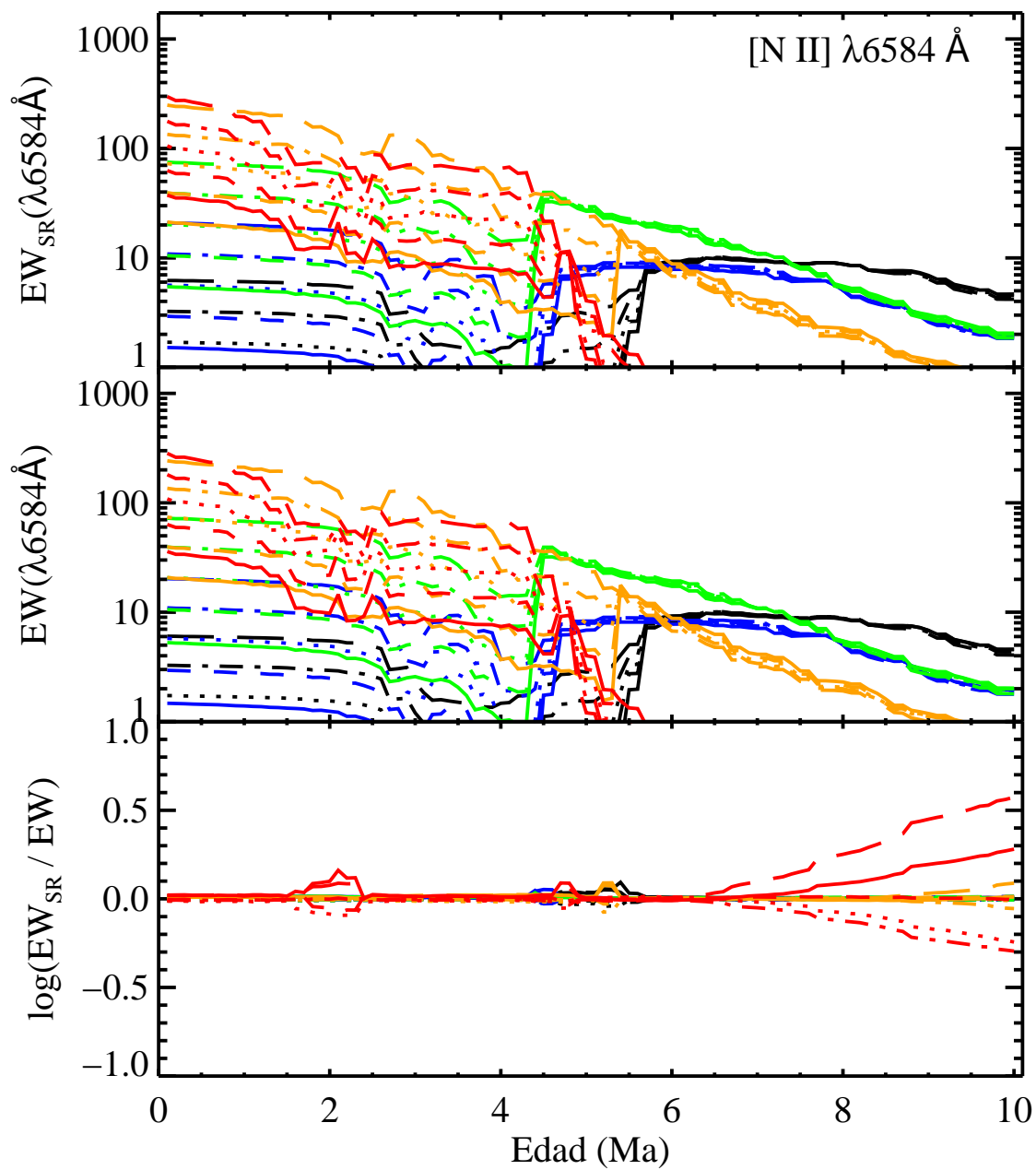
FIGURA C.18: EW_{SR} , EW y \log \frac{EW_{SR}}{EW} para [N II] \lambda 6584 Å.
