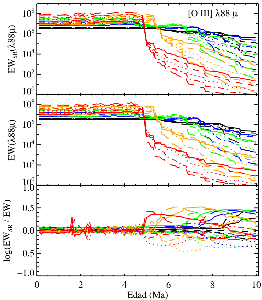
FIGURA C.37: EW_{SR} , EW y \log \frac{EW_{SR}}{EW} para [O III] \lambda 88 \mu .
