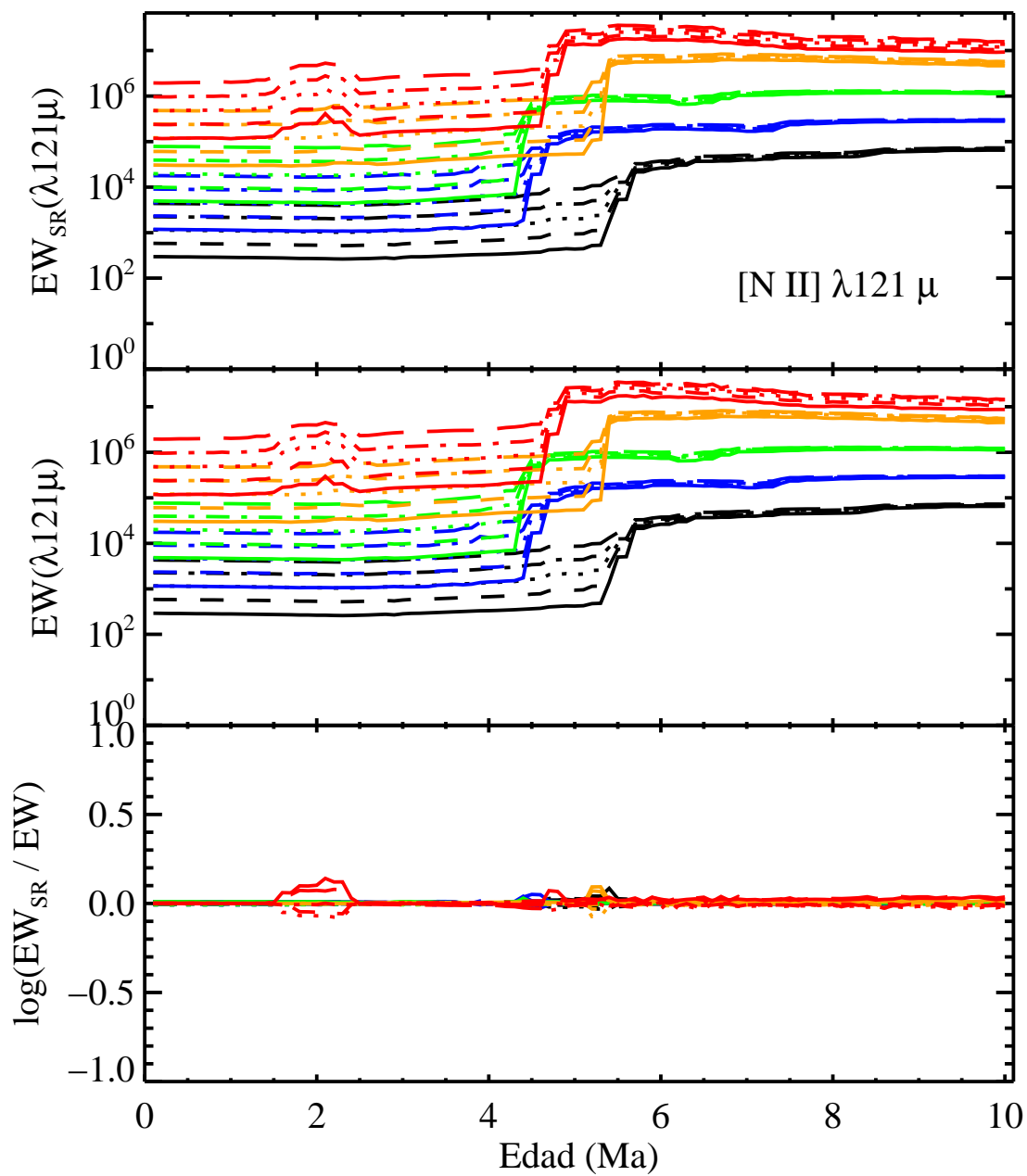
FIGURA C.38: [ EW_{SR} , EW y \log \frac{EW_{SR}}{EW} para [N II] \lambda 121 \mu .
