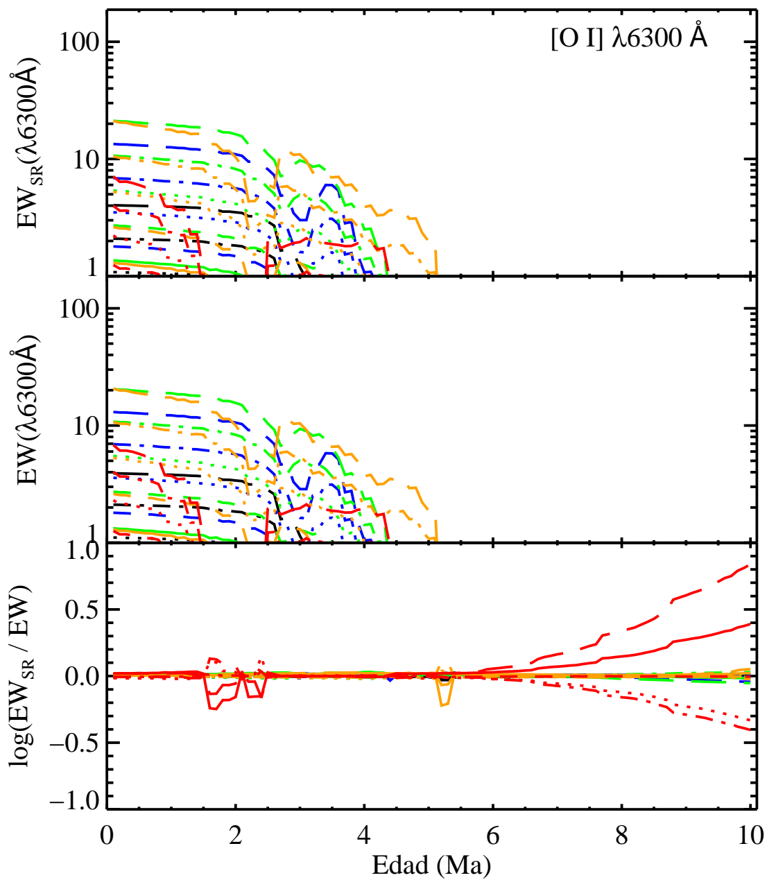
FIGURA C.14: EW_{SR} , EW y \log \frac{EW_{SR}}{EW} para [O \text{ I}] \lambda 6300 \text{ \AA} .
