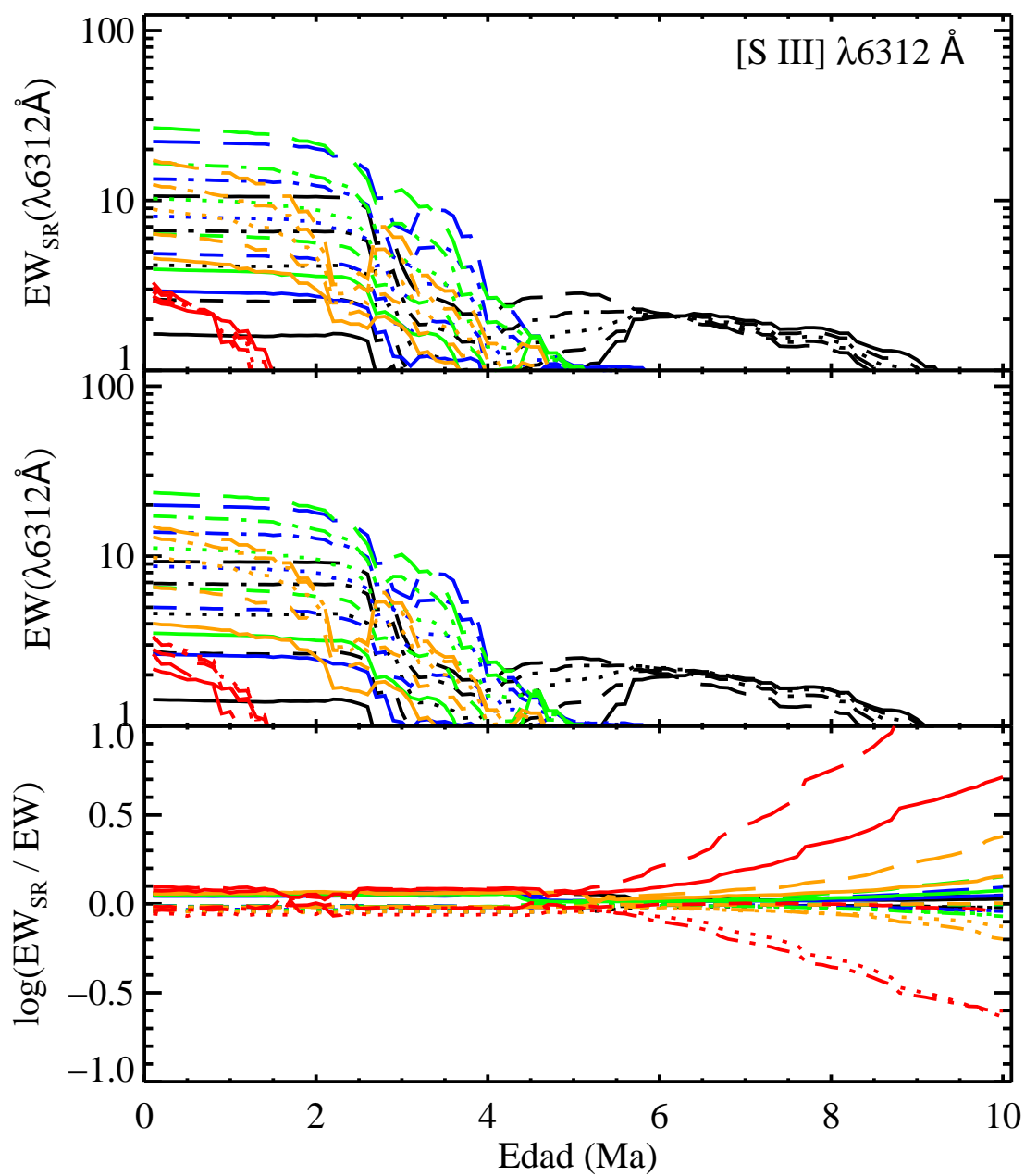
FIGURA C.15: EW_{SR} , EW y \log \frac{EW_{SR}}{EW} para [S III] \lambda 6312 Å.
