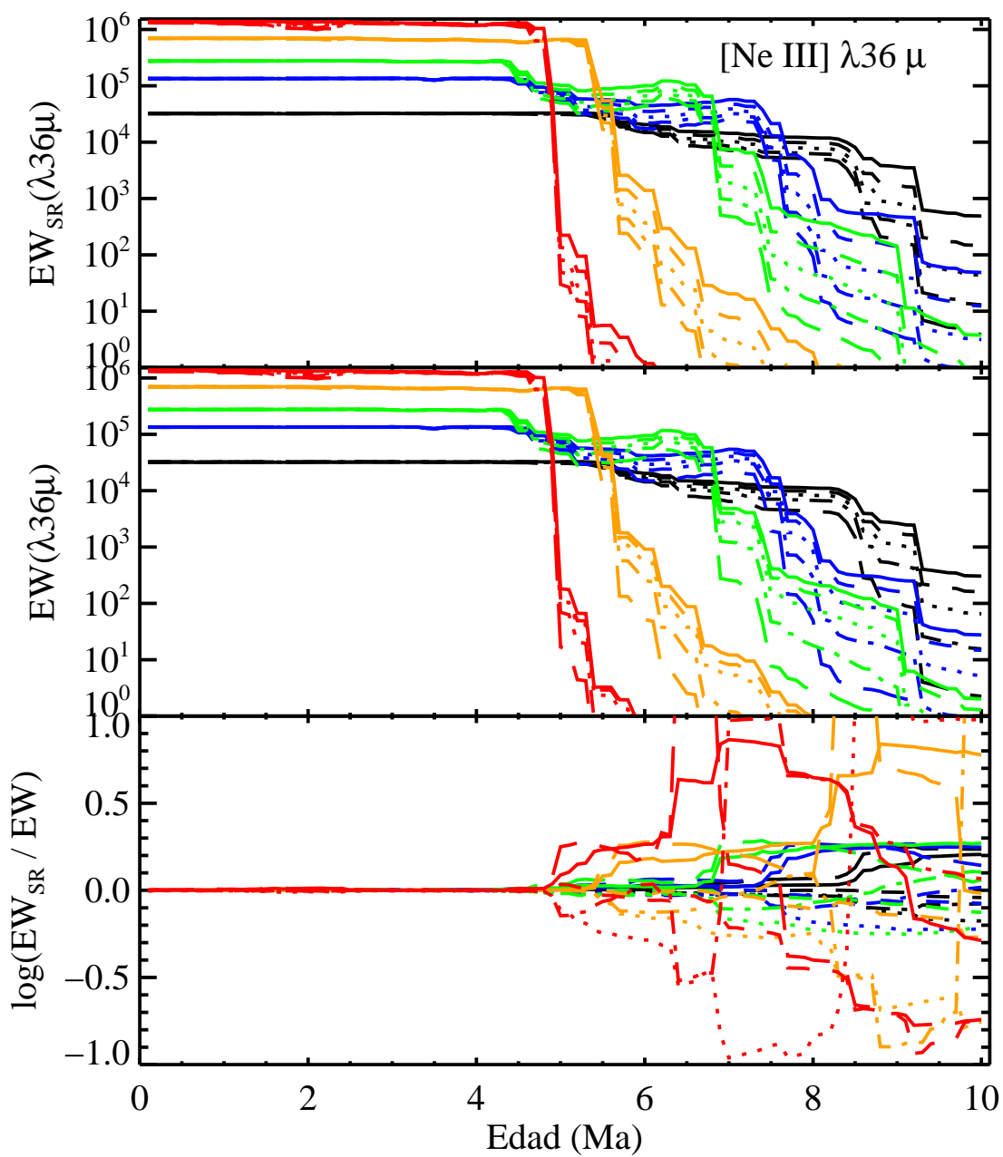
FIGURA C.34: EW_{SR} , EW y \log \frac{EW_{SR}}{EW} para [Ne III] \lambda 36 \mu .
