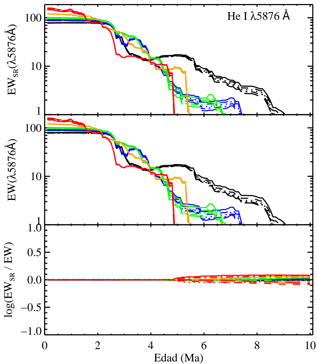
FIGURA C.13: EW_{SR} , EW y \log \frac{EW_{SR}}{EW} para He I \lambda 5876 \text{ \AA} .
